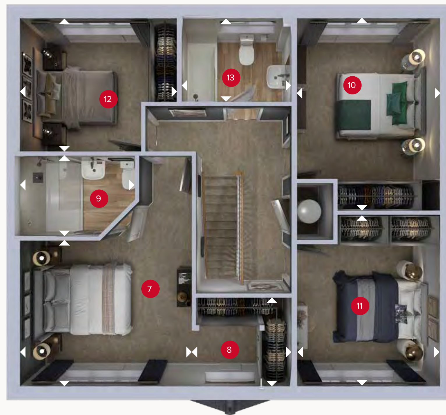
FIRST FLOOR
